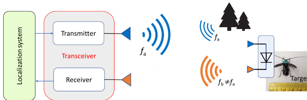
Nonlinear radar system
