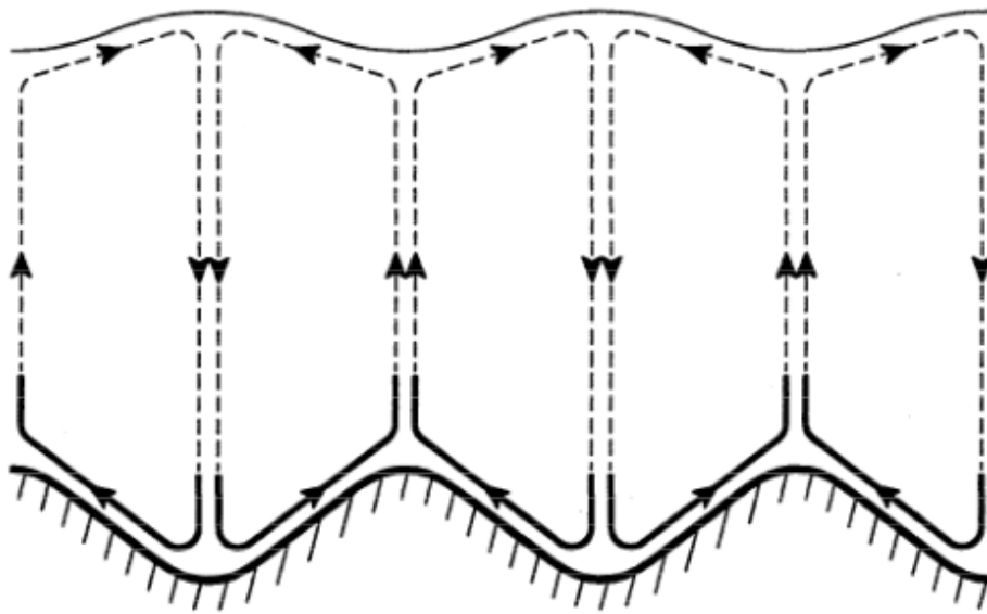
Figure 3 Recirculating cells due to the interaction of a symmetric oscillatory tidal current with sand waves (Hulscher, 1996).
