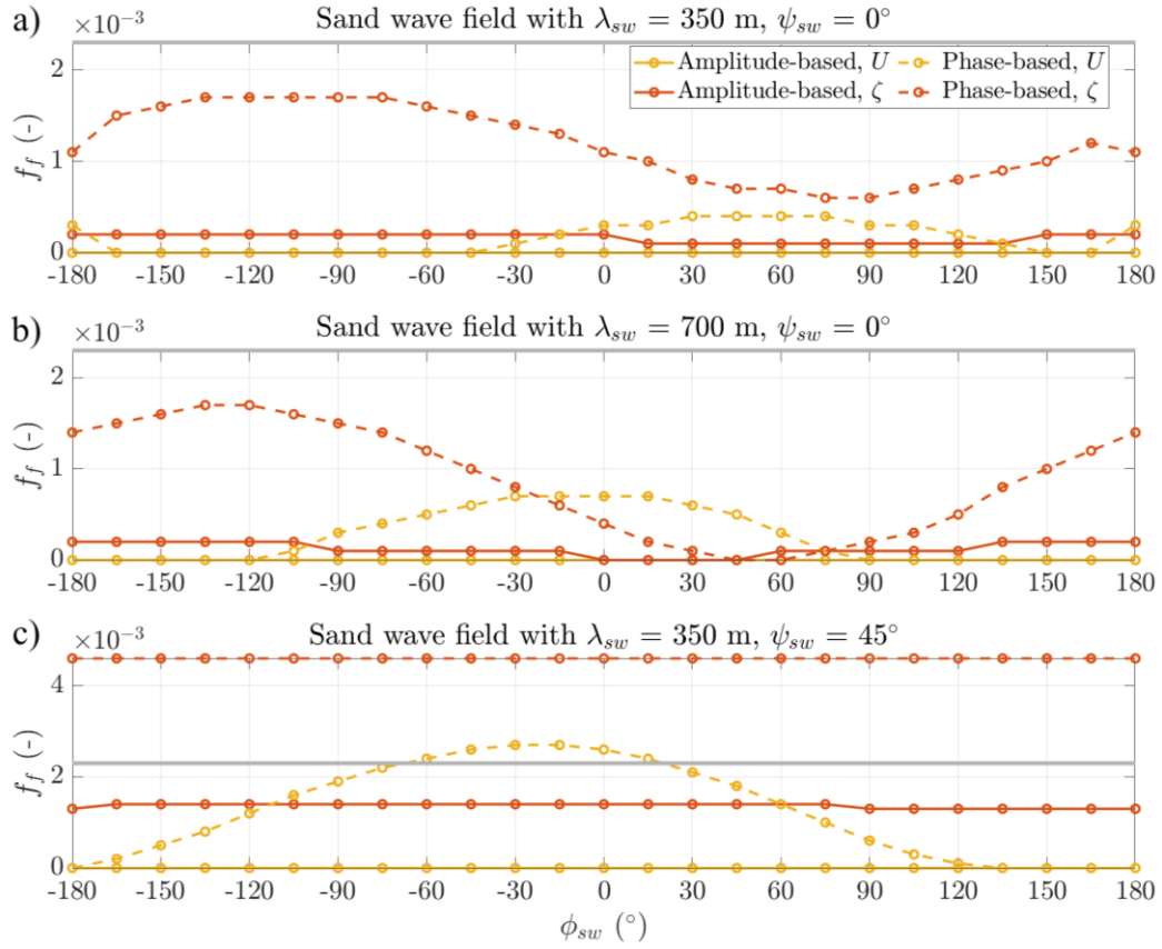
Figure 22 Form roughness ( f_f ) for a sand wave field with different characteristics across different phase angles ( \phi_{sw} ): (a) \lambda_{sw} = 350 m – \psi_{sw} = 0^\circ , (b) \lambda_{sw} = 700 m – \psi_{sw} = 0^\circ , (c) \lambda_{sw} = 350 m – \psi_{sw} = 45^\circ . The grey line corresponds to the grain roughness ( f_g ).
