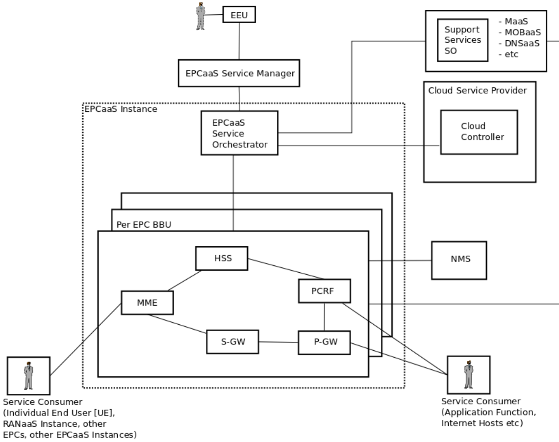
Figure 1.5: EPCaaS architecture reference model, based on [4]
