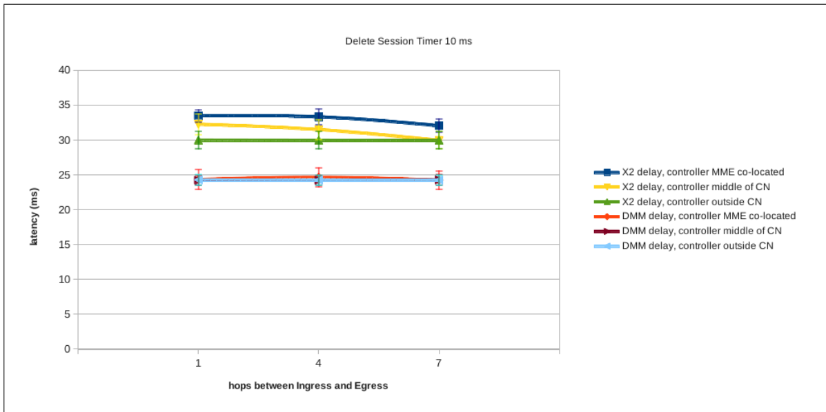
Figure 5.11: Average latency of downlink data packets delivered via X2 path and of the first packets redirected through Partial OpenFlow-based DMM transport network
