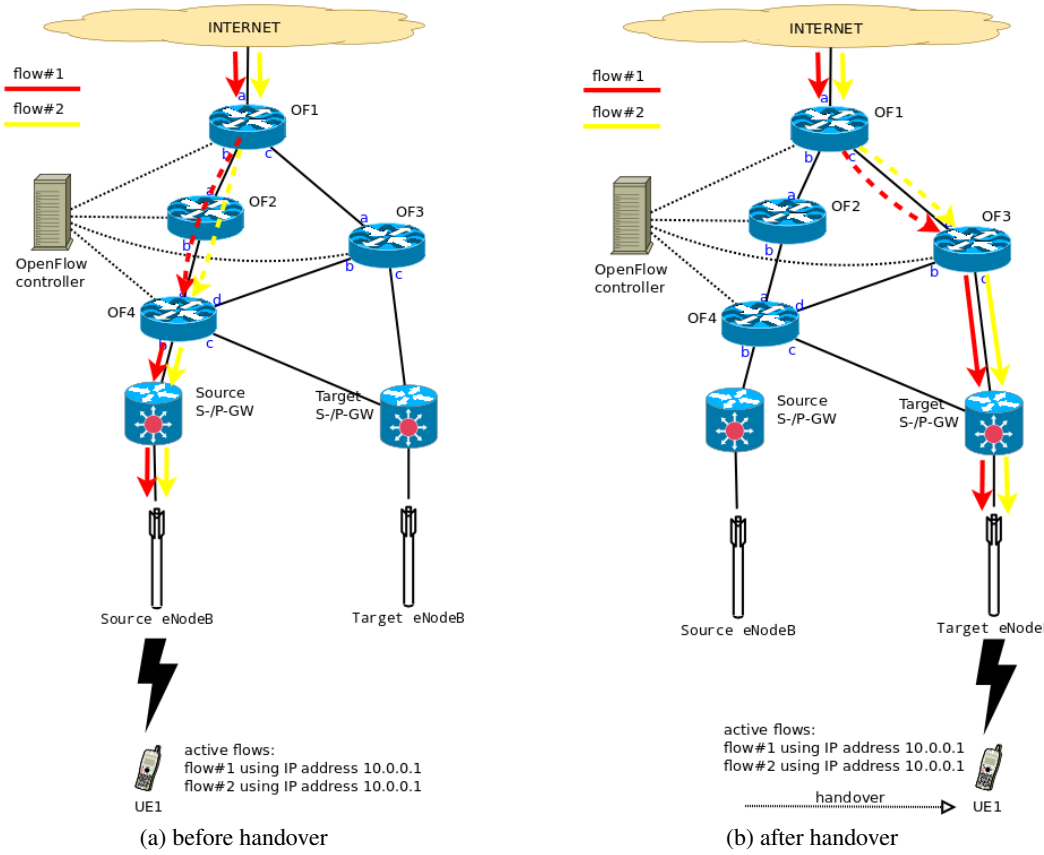
Figure 3.6: Full OpenFlow transport network: downlink per-anchor point flow forwarding
