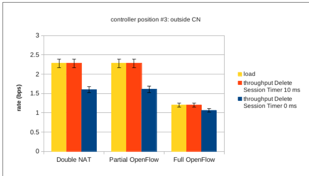
Figure 5.27: Comparison of X2 tunnel throughput with DMM Controller positioned outside of the operator's core network when Double NAT, Partial OpenFlow or Full OpenFlow is used as DMM solution
