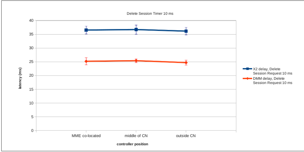
Figure 5.20: Average latency of downlink data packet delivered via X2 path and of the first packets redirected through Full OpenFlow-based DMM transport network
