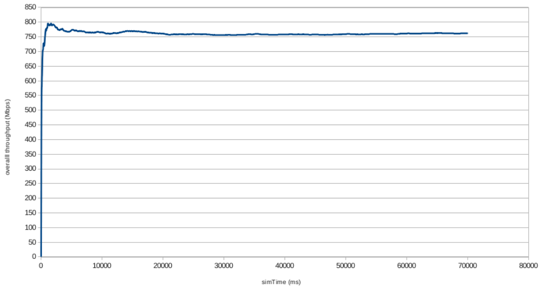
Figure 4.12: Overall throughput growth on a 1 Gbps using NS3 PPBP application
