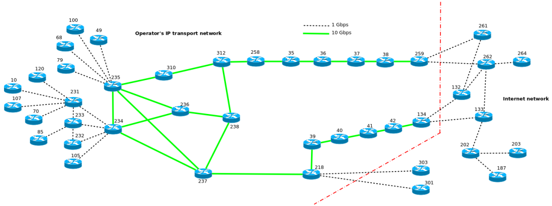
Figure 4.5: Modified simulation IP transport network topology
