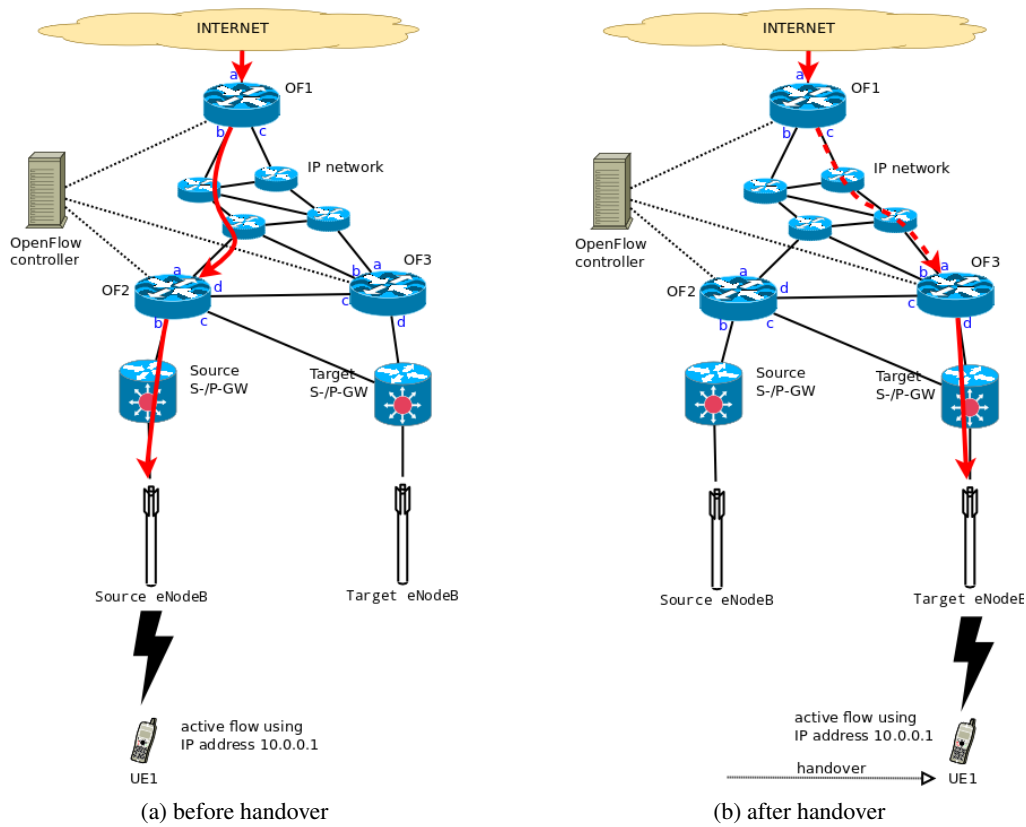
Figure 3.8: Partial OpenFlow transport network downlink flow forwarding
