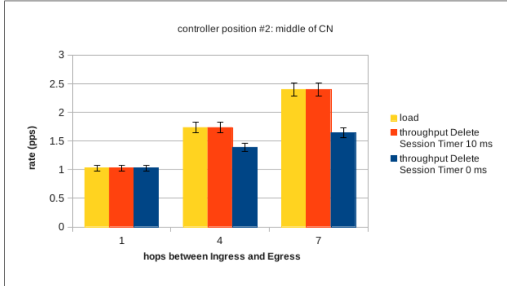
Figure 5.5: Load and throughput of X2 tunnel with NAT Controller positioned in the middle of the core network
