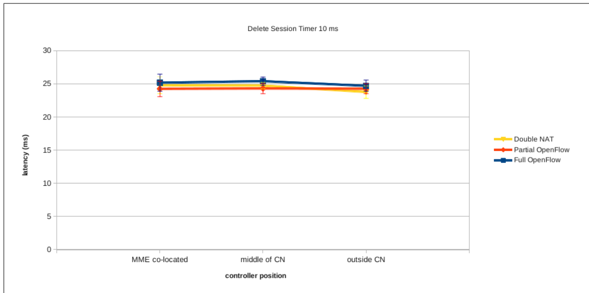
Figure 5.24: Comparison of average latency of downlink data packets delivered via DMM traffic redirection when Double NAT, Partial OpenFlow or Full OpenFlow is used as DMM solution
