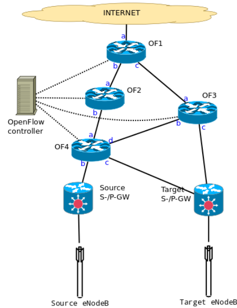
Figure 3.4: Full OpenFlow transport network
