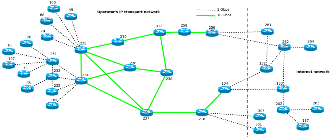
Figure 4.4: Simulation IP transport network topology
