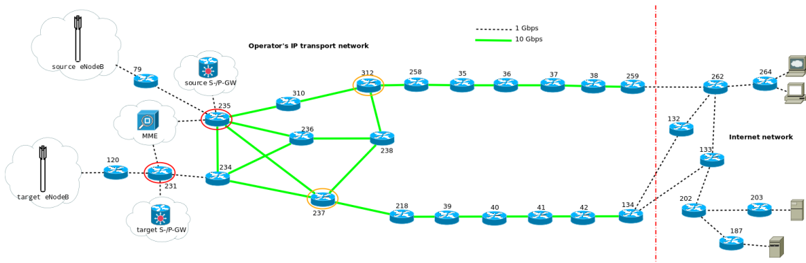
Figure 4.6: First simulation network topology with virtualized LTE-EPC entities: DMM Ingress and Egress points close to the EPC part of the network
