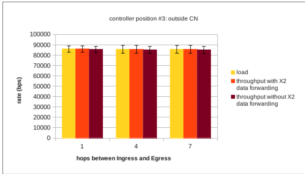
Figure 5.9: Load and total throughputs of the system with and without X2 data forwarding capabilities with NAT Controller positioned outside of the operator's transport network
