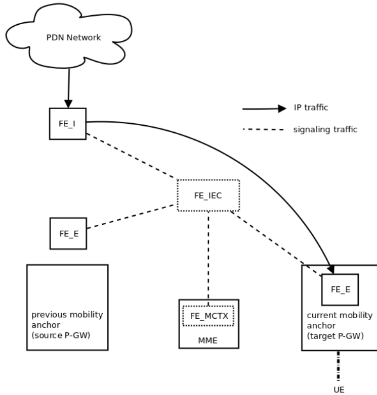
Figure 2.3: Functional entities architecture without IP tunneling
