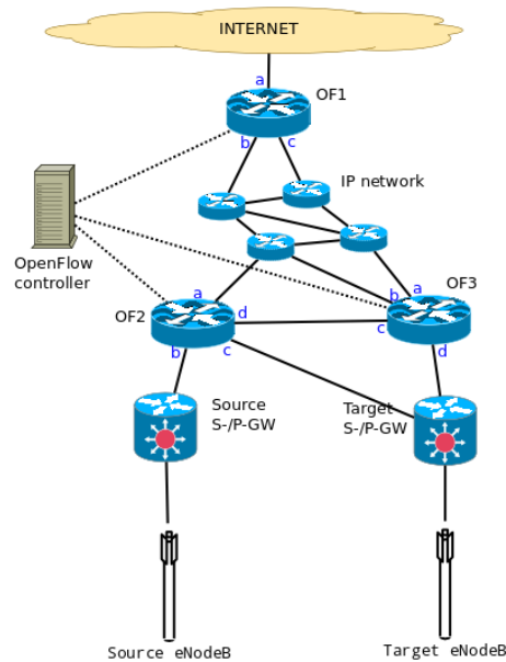
Figure 3.7: Partial OpenFlow transport network
