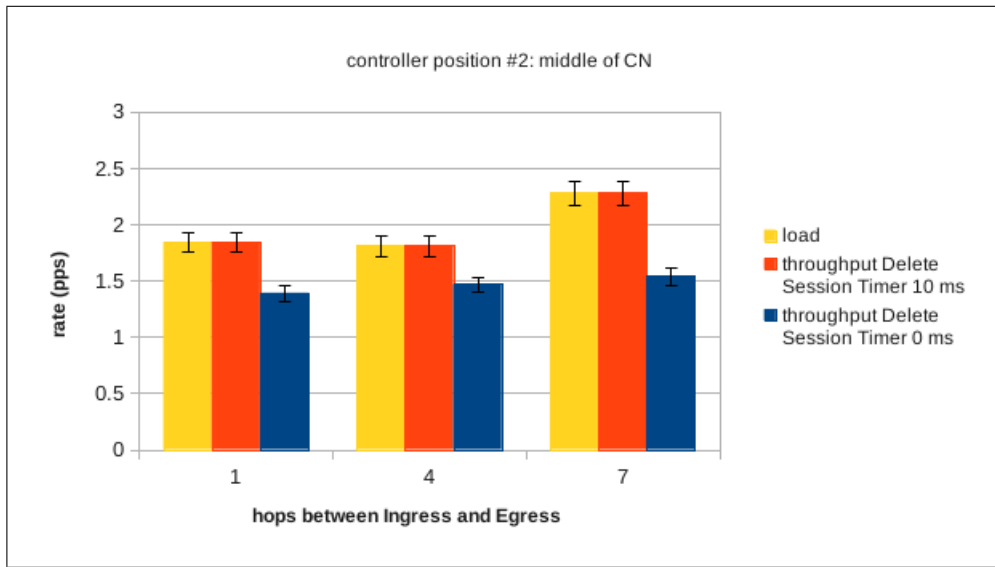
Figure 5.14: Load and throughput of X2 tunnel with OpenFlow Controller positioned in the middle of the core network (Partial OpenFlow)
