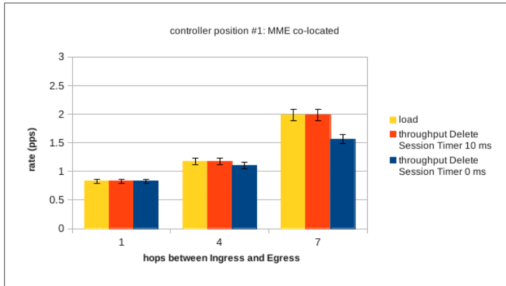
Figure 5.4: Load and throughput of X2 tunnel with NAT Controller co-located with MME
