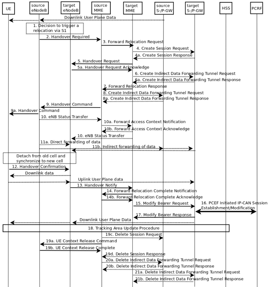
Figure 2.6: S1-based handover with S-/P-GW relocation
