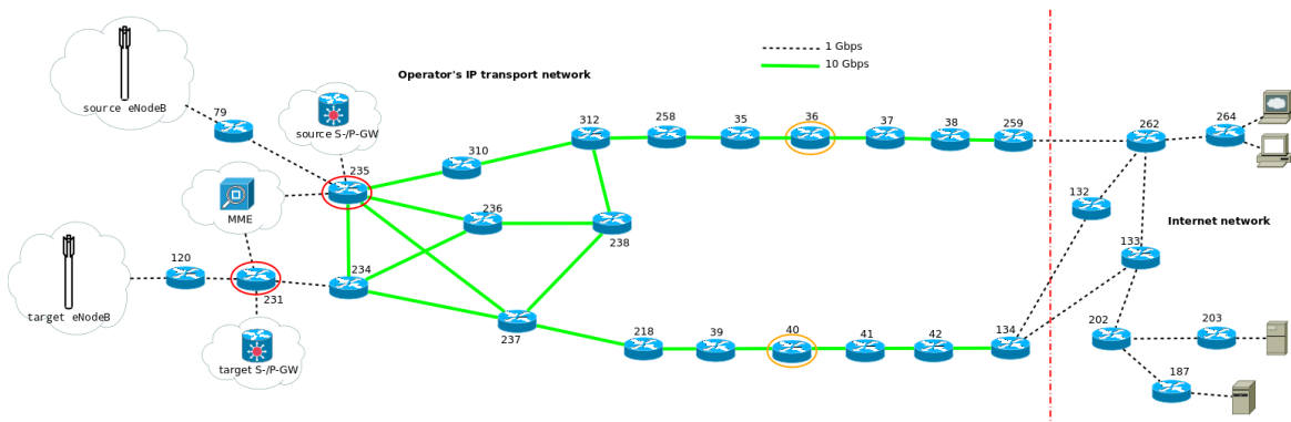
Figure 4.7: Second simulation network topology with virtualized LTE-EPC entities: DMM Ingress placed deeper in the core network
