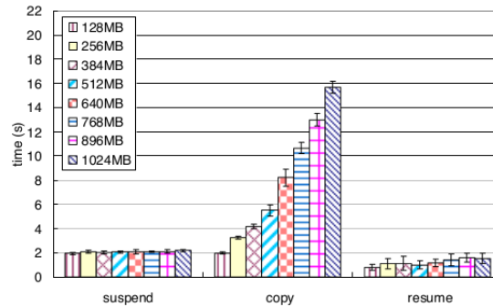
Figure 4.15: The time needed for the three phases of migrating a single VM with different memory sizes, copied from [7]
