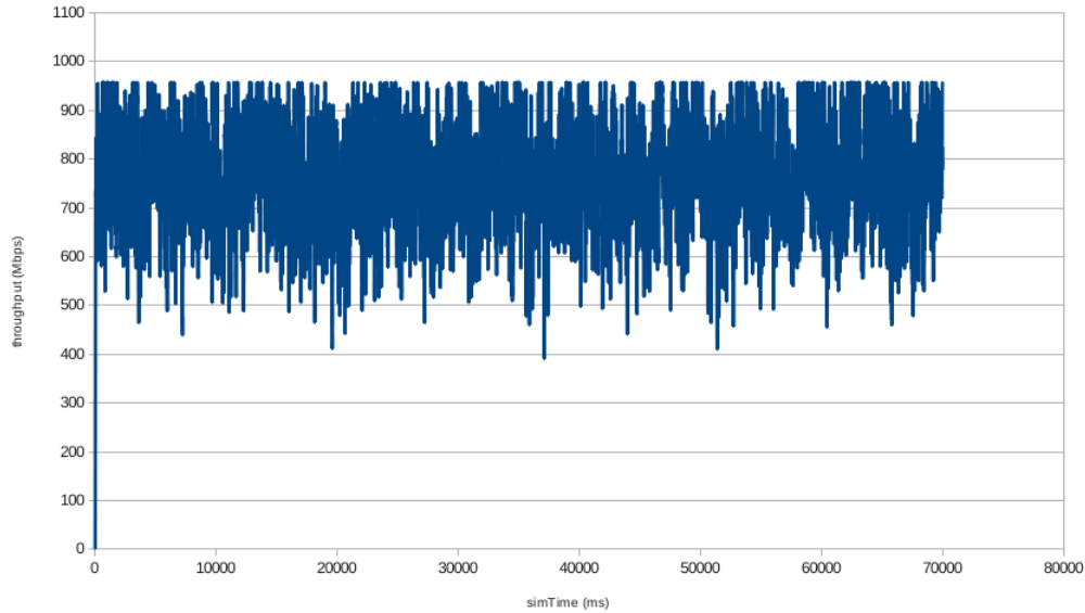
Figure 4.11: Throughput fluctuation on a 1 Gbps using NS3 PPBP application
