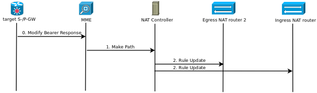
Figure 3.2: Message flow to establish a new downlink path upon reception of a Modify Bearer Response message during handover with S-/P-GW relocation procedure
