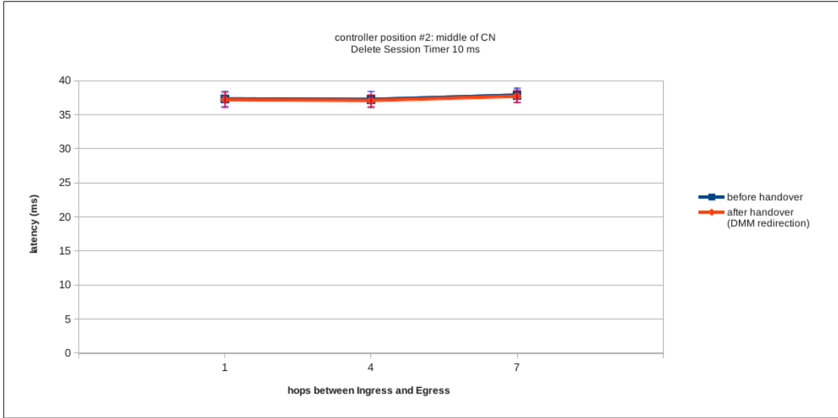
Figure 5.1: Average latency of downlink data packet delivery before and after handover. Double NAT used to redirect the traffic after handover.
