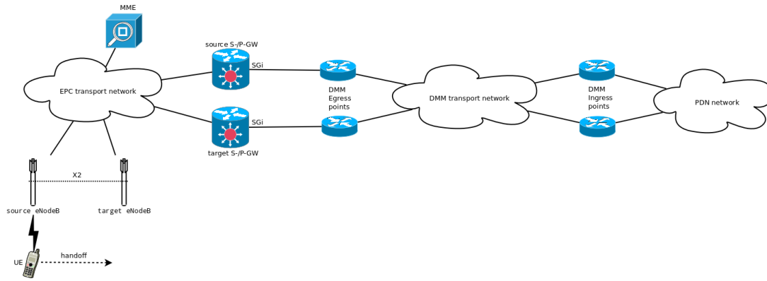
Figure 4.3: Logical simulation topology
