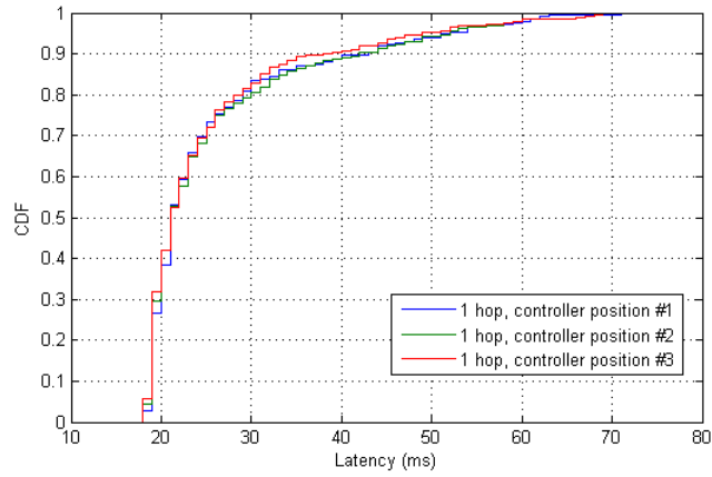
Figure 5.21: CDF of latency of first downlink data packets redirected through Full OpenFlow-based DMM transport network
