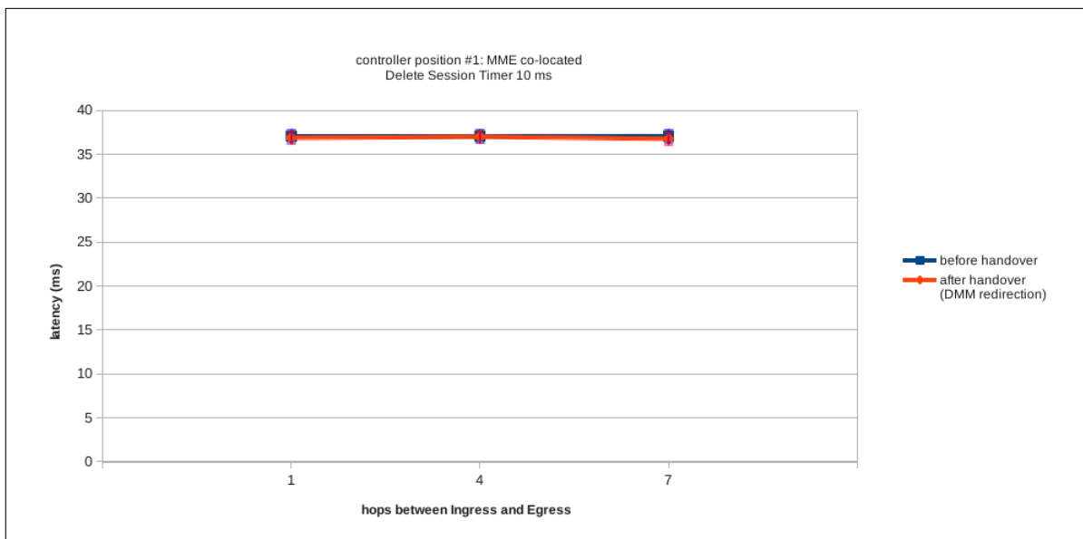
Figure 5.10: Average latency of downlink data packet delivery before and after handover. Partial OpenFlow used to redirect traffic after handover
