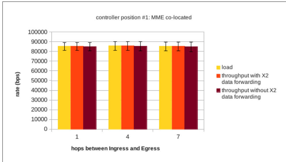
Figure 5.7: Load and total throughputs of the system with and without X2 data forwarding capabilities with NAT Controller co-located with the MME
