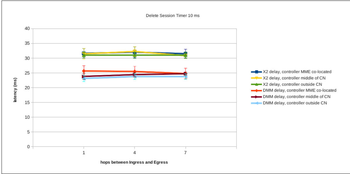
Figure 5.2: Average latency of downlink data packets delivered via X2 path and of the first packet redirected through Double NAT-based DMM transport network
