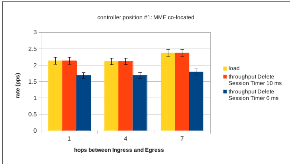
Figure 5.13: Load and throughput of X2 tunnel with OpenFlow Controller co-located with MME (Partial OpenFlow)
