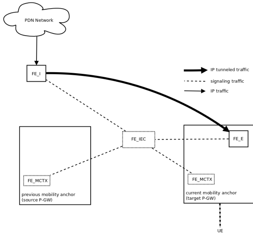
Figure 2.2: Distributed Architecture
