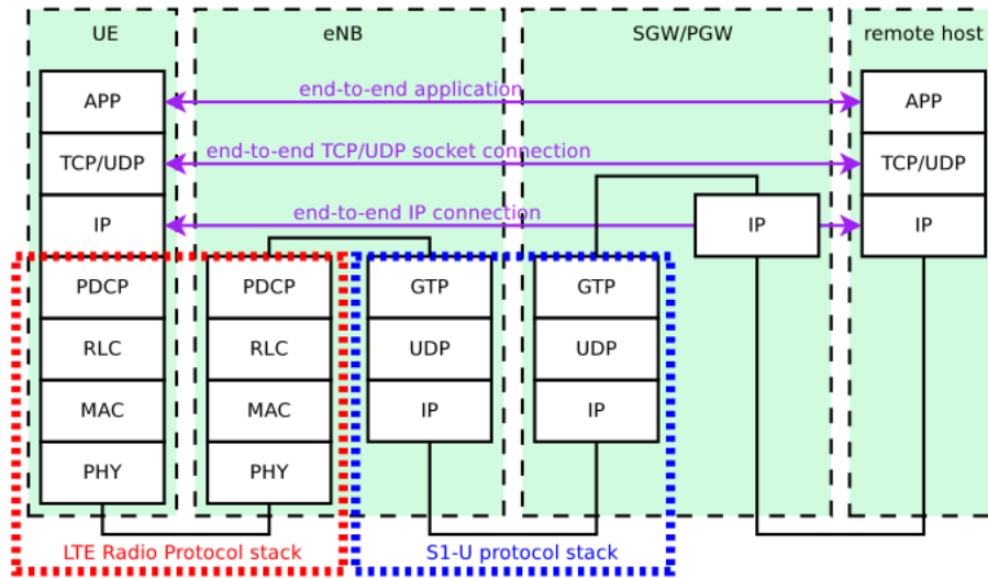
Figure 4.2: NS3 LENA's LTE-EPC data plane protocol stack, copied from [6]
