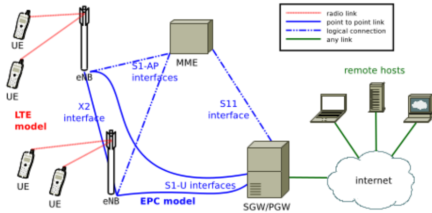
Figure 4.1: Overview of NS3 LENA's LTE-EPC simulation model, copied from [6]
