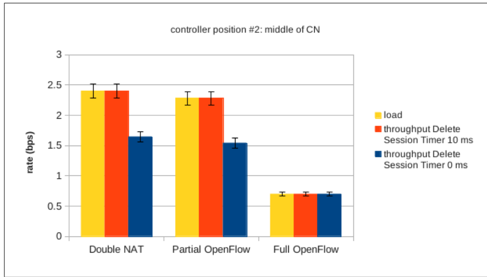
Figure 5.26: Comparison of X2 tunnel throughput with DMM Controller positioned in the middle of the core network when Double NAT, Partial OpenFlow or Full OpenFlow is used as DMM solution
