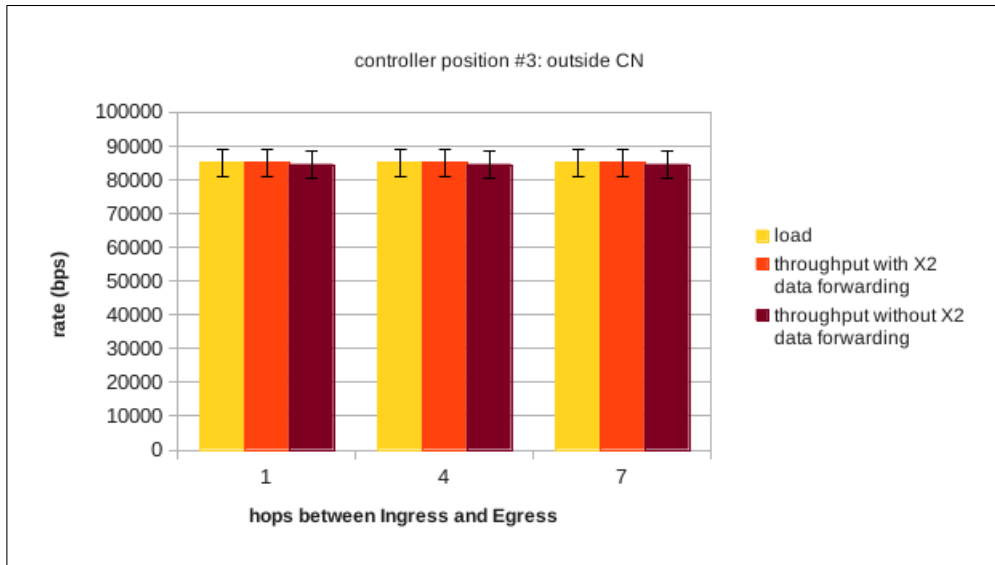
Figure 5.18: Load and total throughputs of the system with and without X2 data forwarding capabilities with OpenFlow Controller positioned outside of the operator's transport network (Partial OpenFlow)
