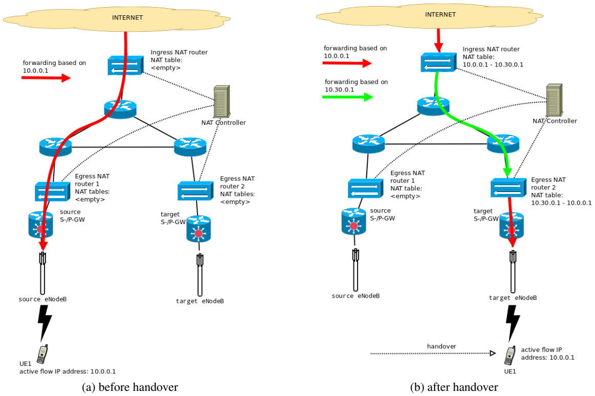
Figure 3.1: Double NAT data plane mechanism
