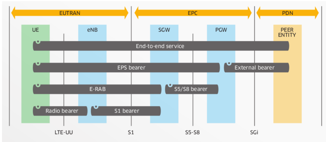
Figure 2.4: Bearer architecture, copied from [5]
