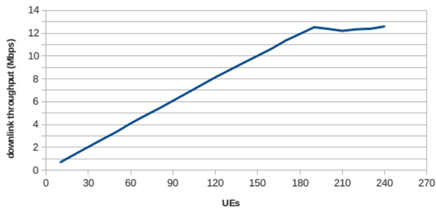
Figure 4.10: eNodeB's downlink throughput growth curve
