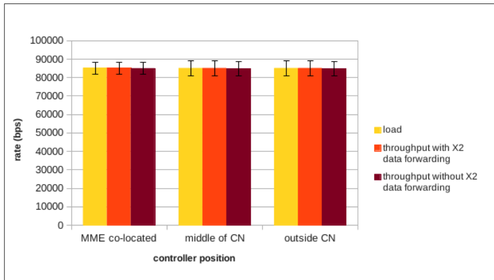
Figure 5.23: Load and throughputs of the system with and without X2 data forwarding capabilities with different OpenFlow Controller positioning (Full OpenFlow)
