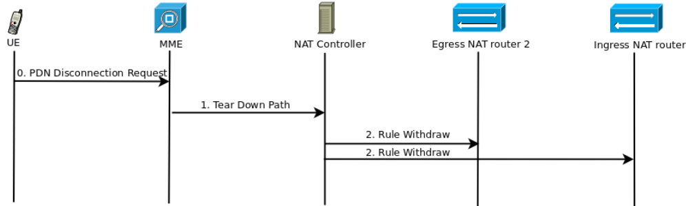
Figure 3.3: Message flow to remove a downlink path upon reception of PDN Disconnection Request from the UE
