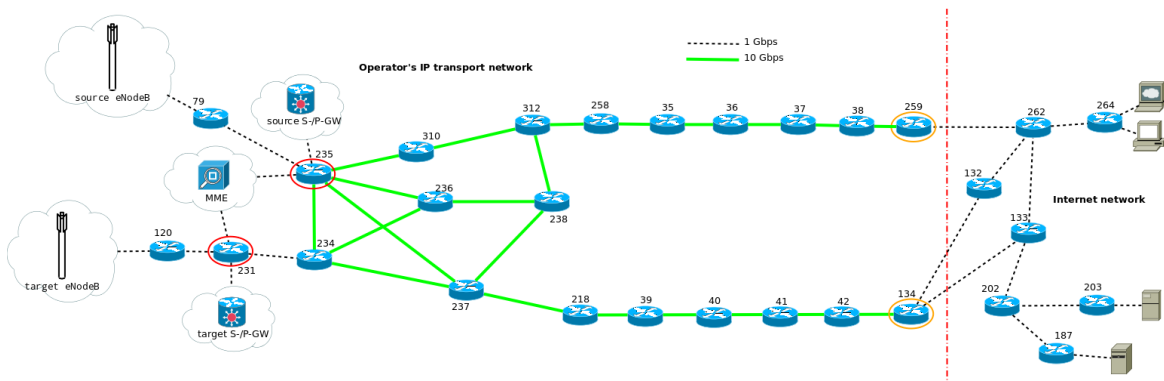
Figure 4.8: Third simulation network topology with virtualized LTE-EPC entities: DMM Ingress and Egress on opposite edges of the operator's network
