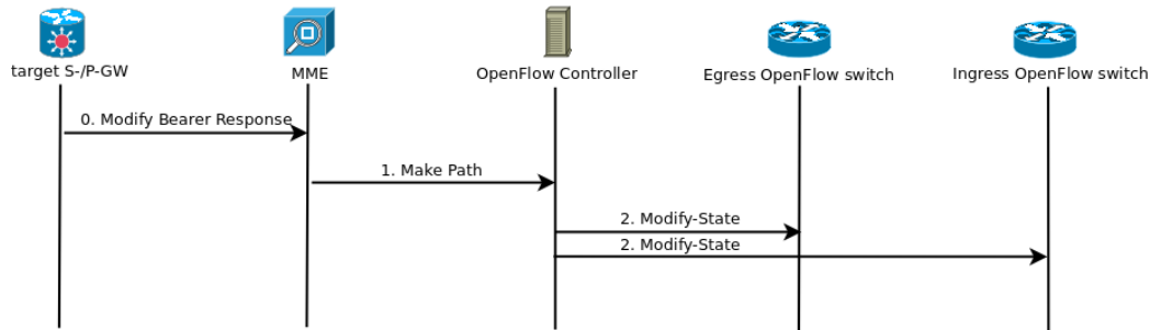
Figure 3.9: Message flow to establish a new downlink path upon reception of a Modify Bearer Response message during handover with S-/P-GW relocation procedure
