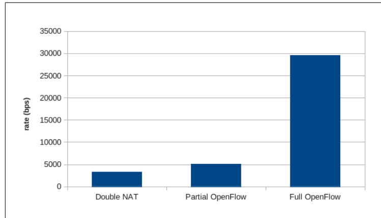
Figure 5.30: Comparison of signaling load of the system when Double NAT, Partial OpenFlow or Full OpenFlow is deployed as DMM solution
