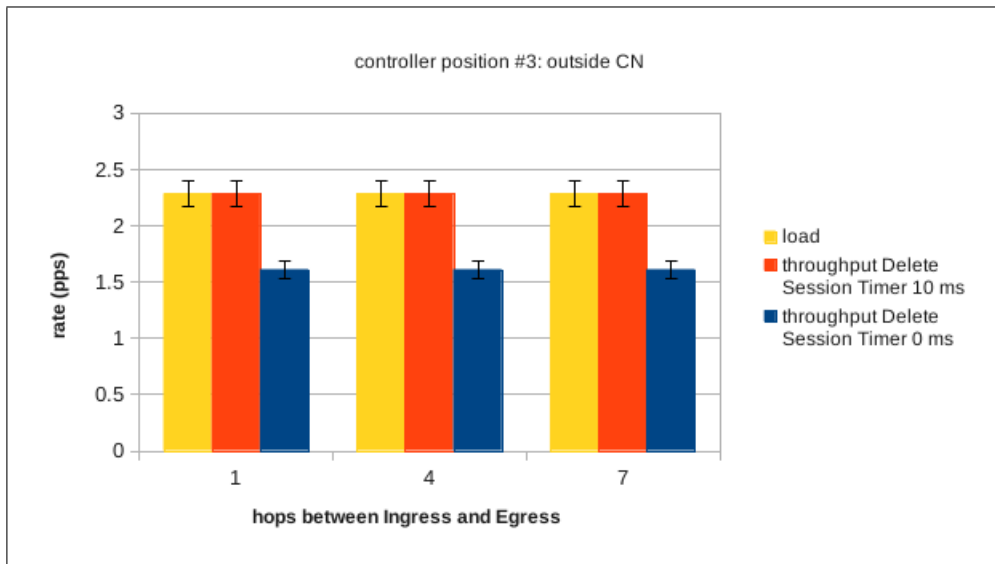
Figure 5.15: Load and throughput of X2 tunnel with OpenFlow Controller positioned outside of the operator's transport network (Partial OpenFlow)
