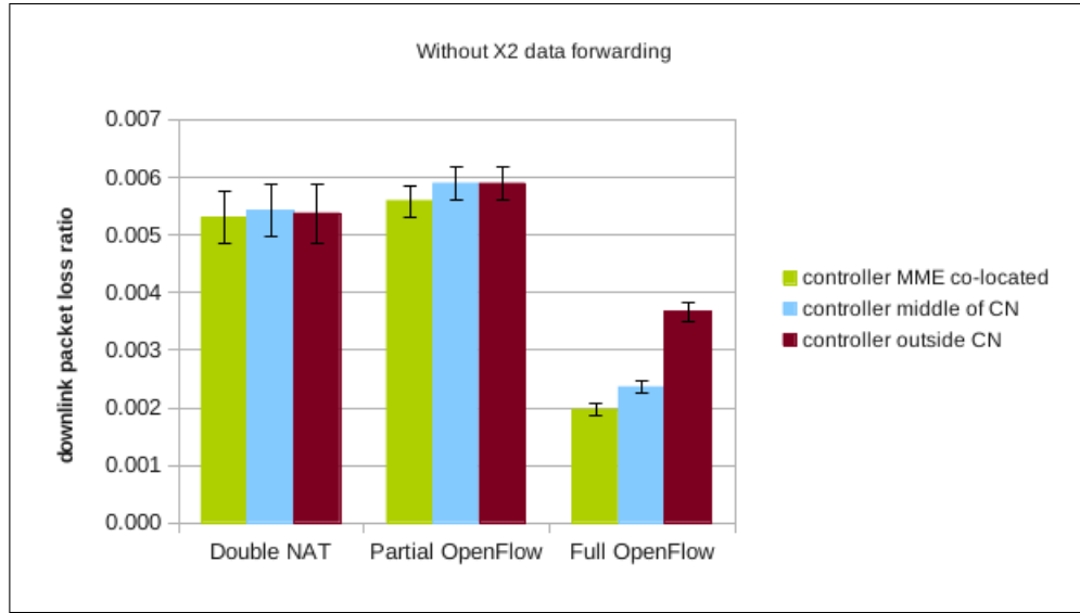
Figure 5.29: Comparison of downlink packet loss ratio of the system when Double NAT, Partial OpenFlow or Full OpenFlow is deployed as DMM solution and no X2 data forwarding capability is present in the network
