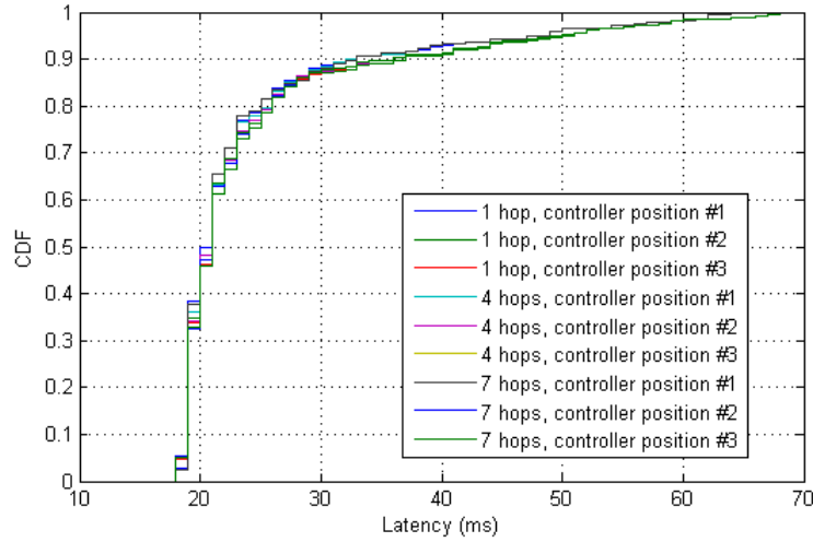
Figure 5.12: CDF of latency of first downlink data packets redirected through Partial OpenFlow-based DMM transport network
