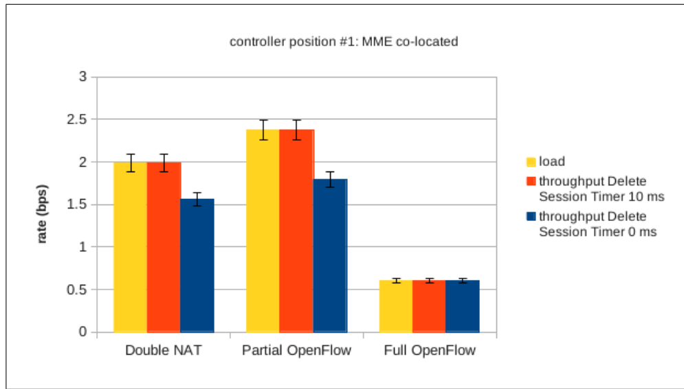
Figure 5.25: Comparison of throughput of X2 tunnel with DMM Controller co-located with MME when Double NAT, Partial OpenFlow or Full OpenFlow is used as DMM solution
