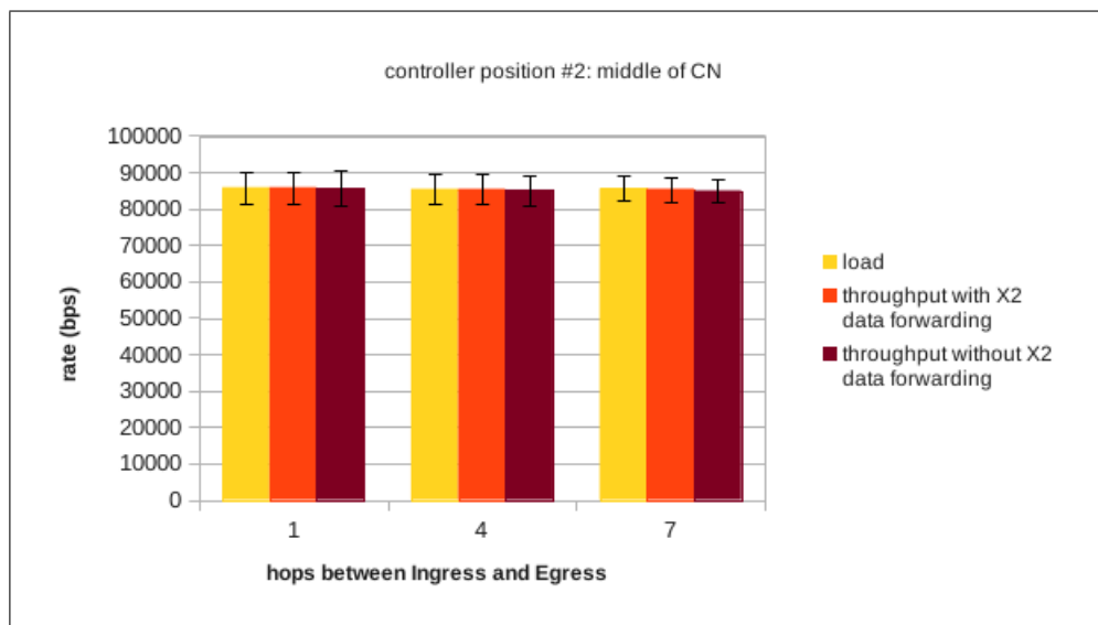
Figure 5.8: Load and total throughputs of the system with and without X2 data forwarding capabilities with NAT Controller positioned in the middle of the core network
