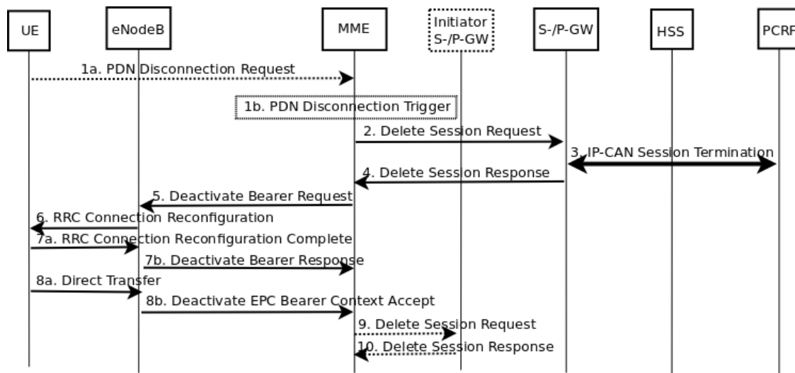
Figure 2.7: UE or MME requested PDN disconnection
