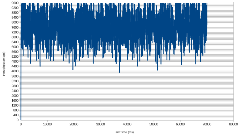
Figure 4.13: Throughput fluctuation on a 10 Gbps using NS3 PPBP application
