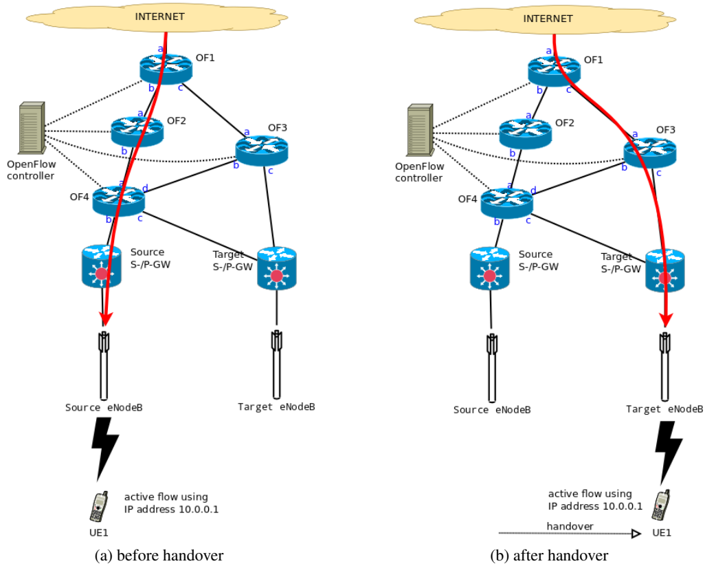
Figure 3.5: Full OpenFlow transport network: downlink per-user flow forwarding
