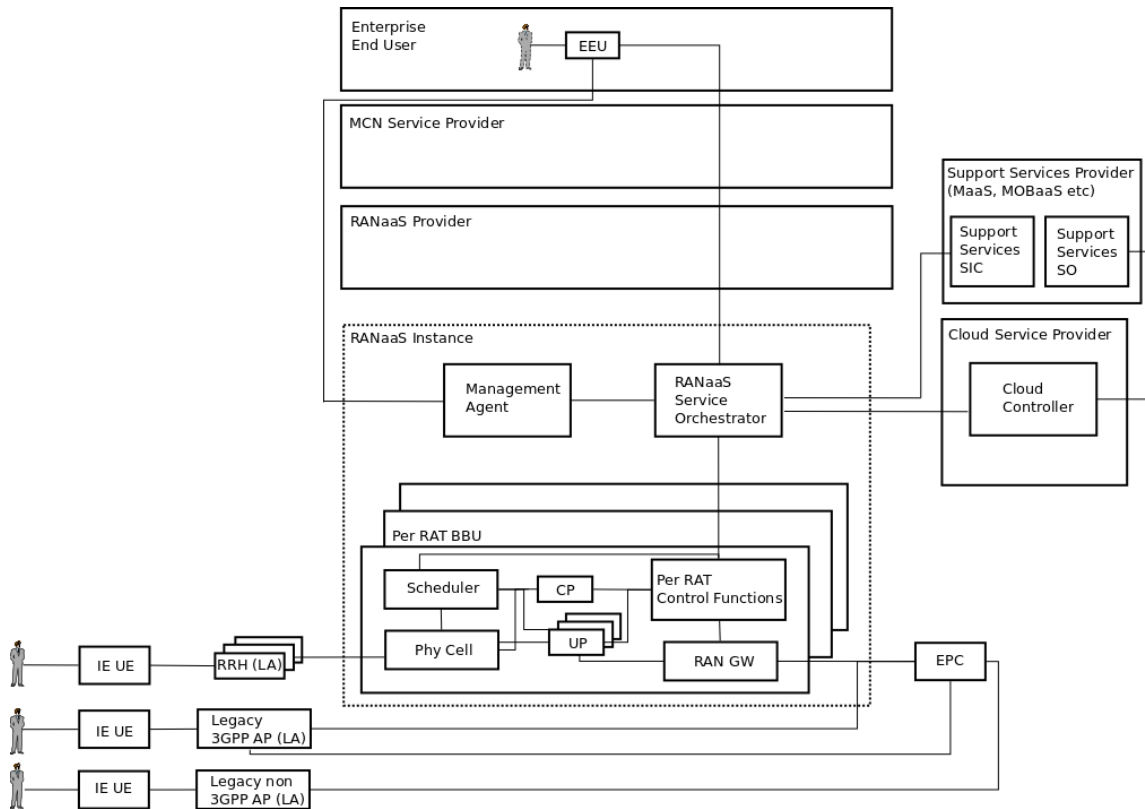
Figure 1.4: RANaaS architecture reference model, based on [4]
