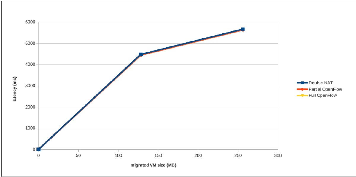
Figure 5.31: Average latency of first downlink data packet received after the completion of the VM migration when Double NAT, Partial OpenFlow or Full OpenFlow is the deployed DMM solution in the network
