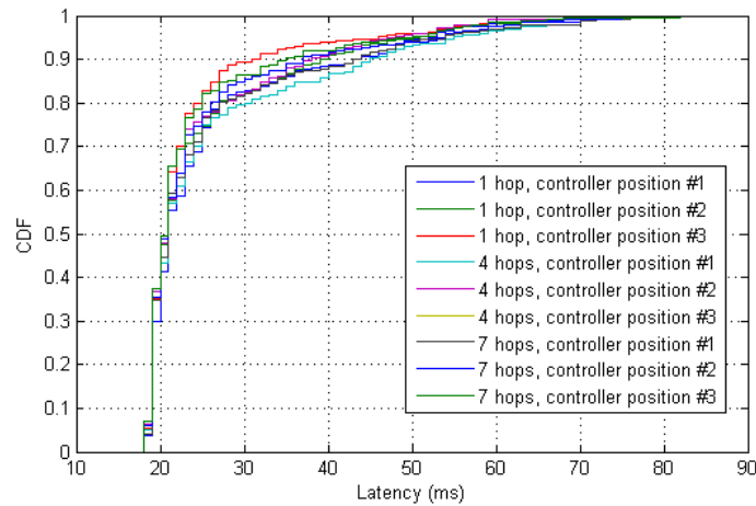
Figure 5.3: CDF of latency of first downlink data packets redirected through Double NAT-based DMM transport network
