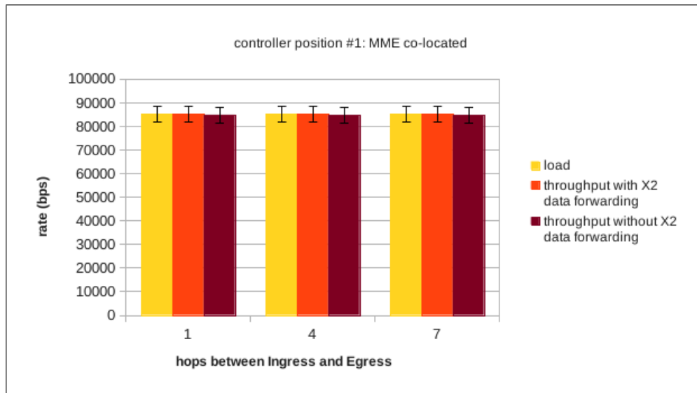
Figure 5.16: Load and total throughputs of the system with and without X2 data forwarding capabilities with OpenFlow Controller co-located with the MME (Partial OpenFlow)
