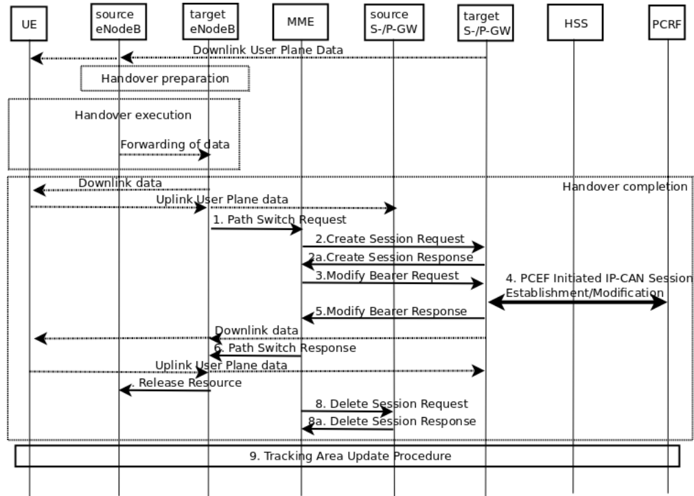
Figure 2.5: X2-based handover with S-/P-GW relocation
