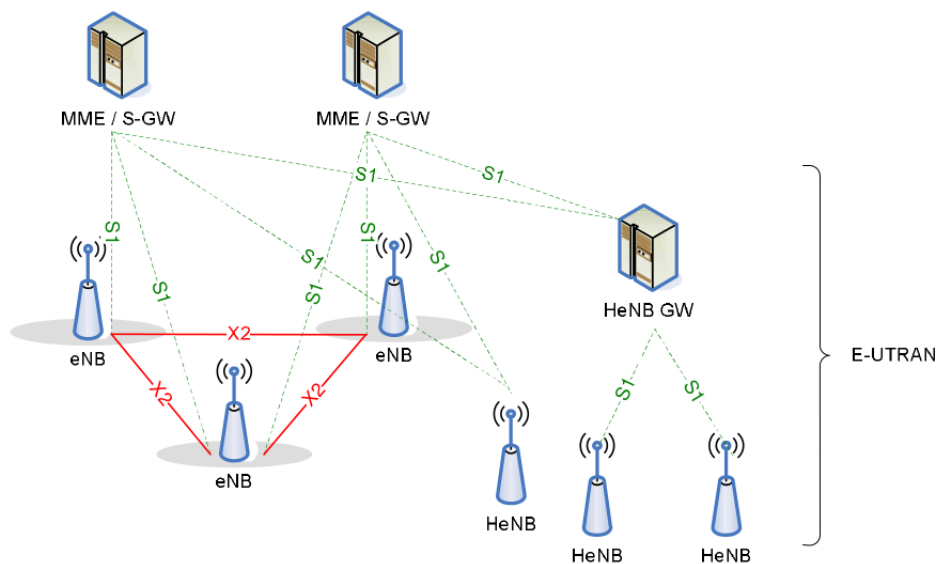
Figure 1.3: Overall E-UTRAN architecture with deployed HeNB, copied from [3]
