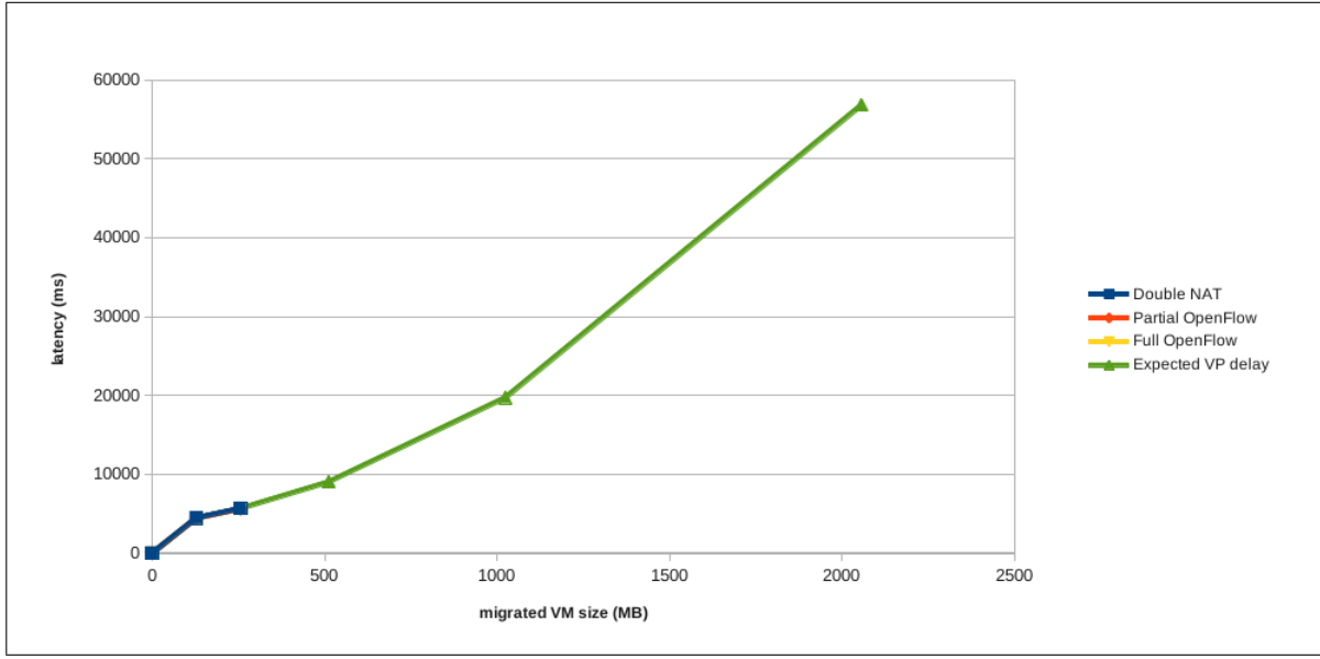
Figure 5.32: Average latency of first downlink data packet received after the completion of the VM migration when Double NAT, Partial OpenFlow or Full OpenFlow is the deployed DMM solution in the network
