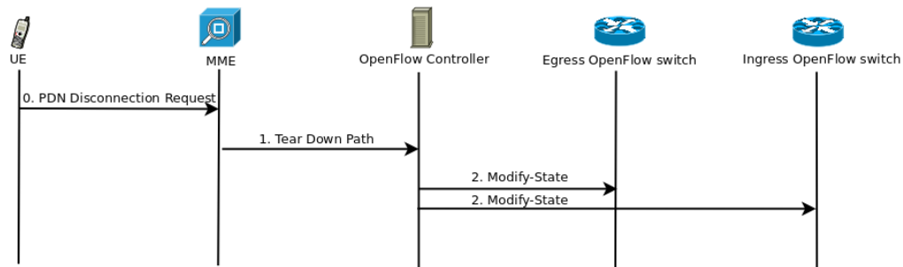
Figure 3.10: Message flow to remove a downlink path upon reception of PDN Disconnection Request from the UE
