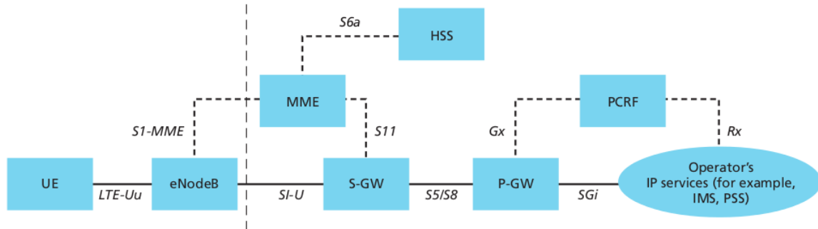
Figure 1.2: The EPS network elements, copied from [2]
