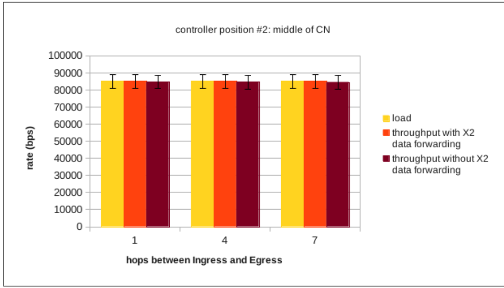
Figure 5.17: Load and total throughputs of the system with and without X2 data forwarding capabilities with OpenFlow Controller positioned in the middle of the core network (Partial OpenFlow)
