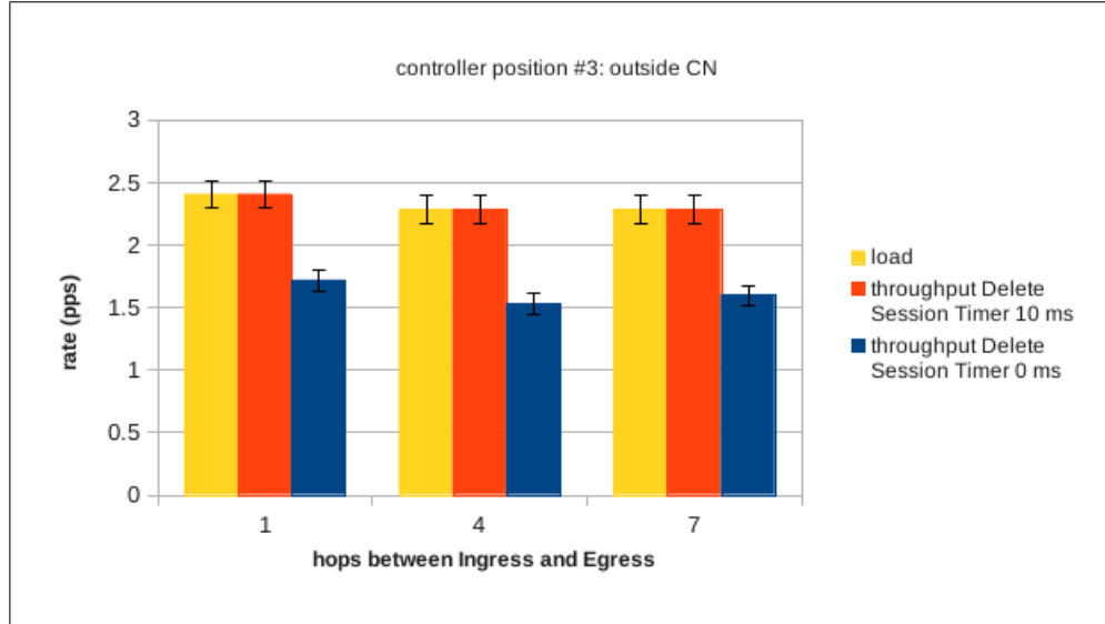
Figure 5.6: Load and throughput of X2 tunnel with NAT Controller positioned outside of the operator's transport network
